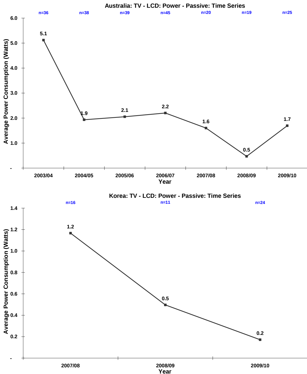
Figure 25 Australian & Korean Time Series Data – LCD TV Passive Mode
