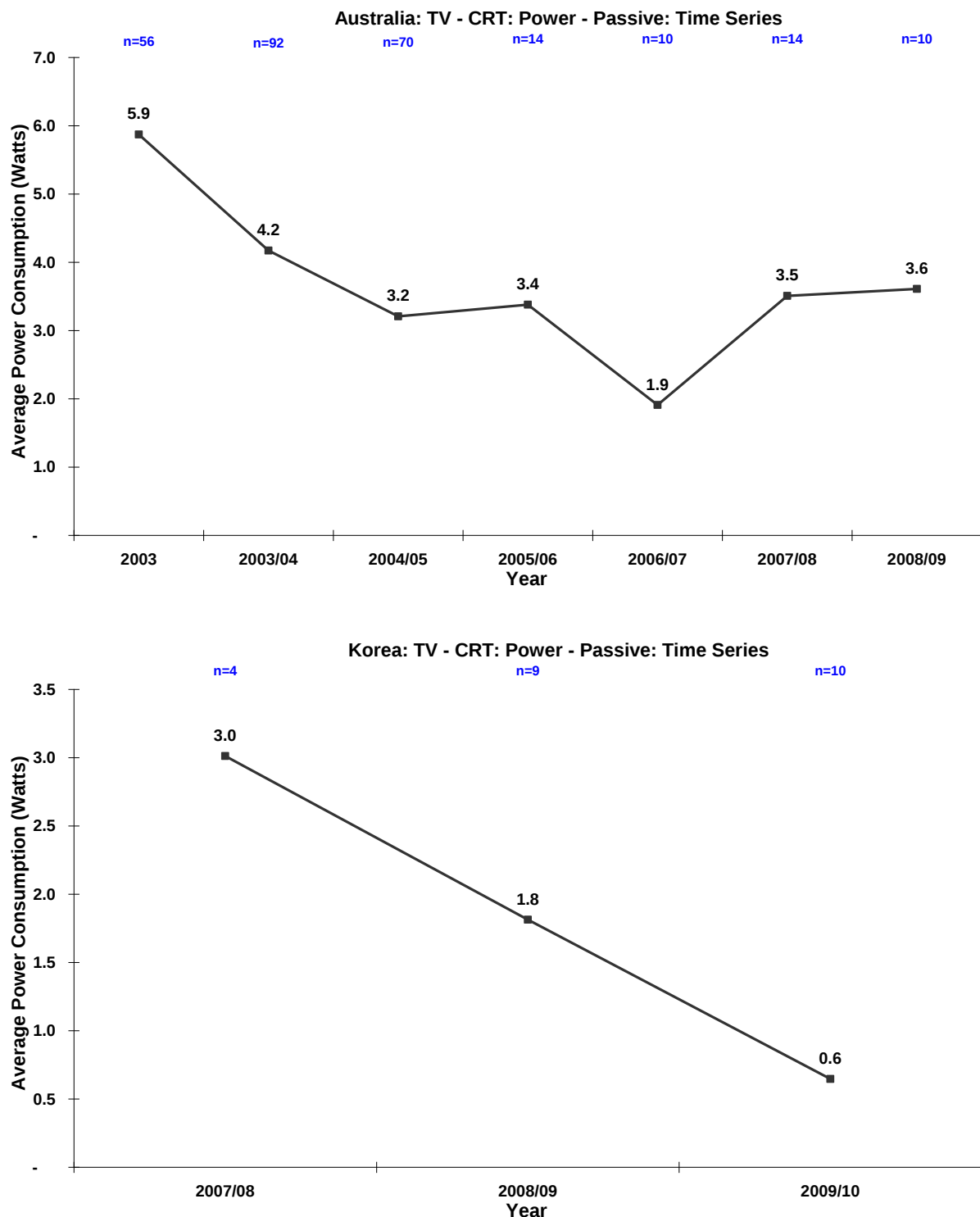
Figure 23 Australian and Korean Time Series Data – CRT TV Passive Mode
