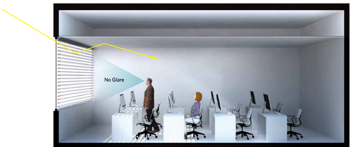
FIGURE 4.5.2 | CROSS-SECTION OF DAYLIGHT HARVESTING FROM FAÇADE USING HORIZONTAL VENETIAN BLINDS
