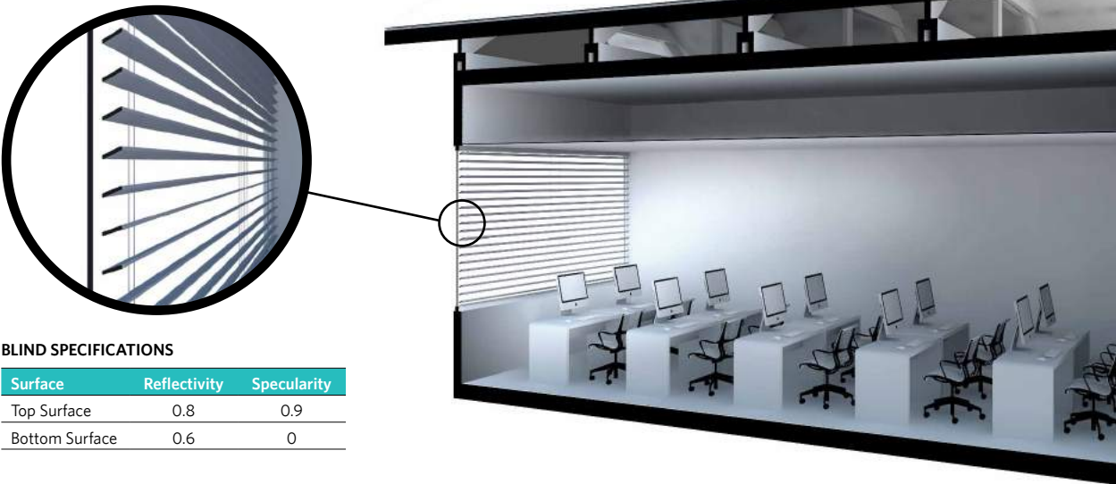
FIGURE 4.5.3 | MODEL OF DAYLIGHT HARVESTING SIMULATION CONDUCTED USING RADIANCE
