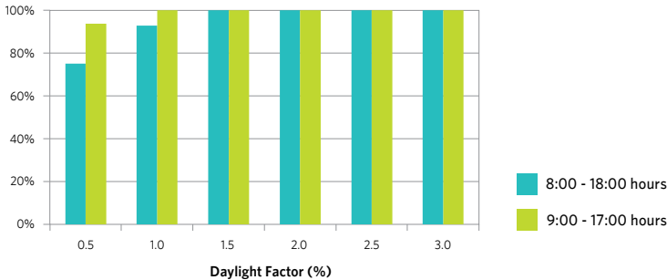
CHART 4.3 | PERCENTAGE OF HOURS WHERE THE DAYLIGHT FACTOR OF DIFFUSE LIGHT EXCEEDS 300 LUX LEVEL
