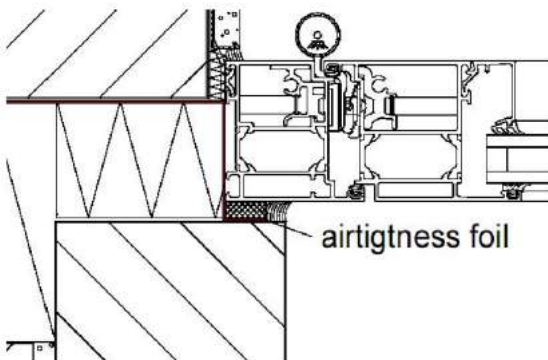
Horizontal section (aluminium door), thermally separated, with air-tightness foil
