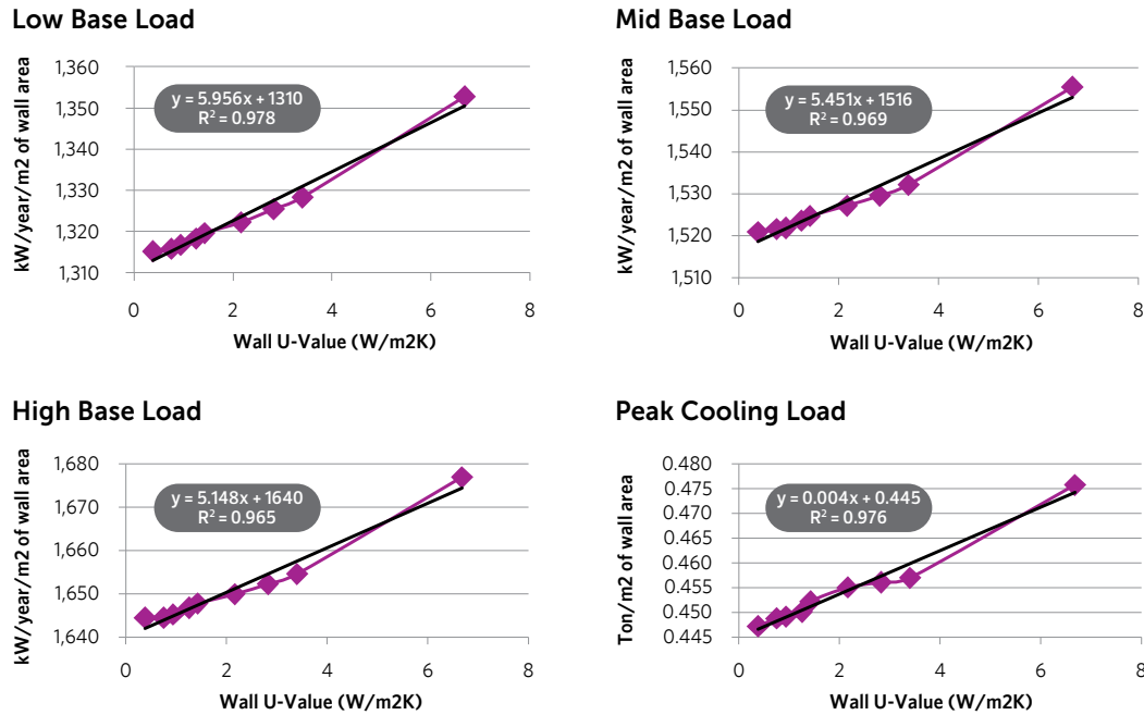
CHART 7.4 | LINEAR CURVE FIT OF ENERGY CONSUMPTION AND PEAK COOLING LOAD IN BUILDING
