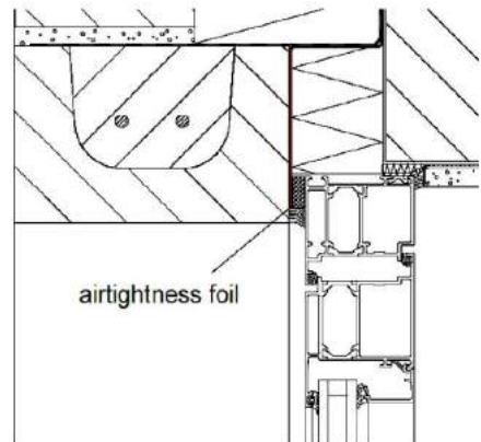
Vertical section (aluminium door), thermally separated, with air-tightness foil
