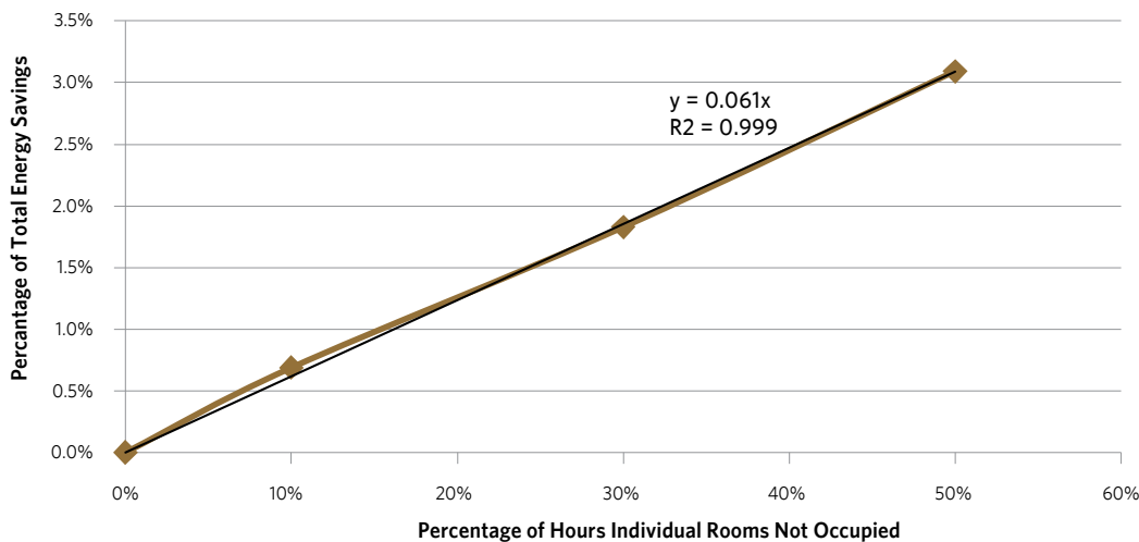
CHART 11.1 | TOTAL BUILDING ENERGY SAVED BY PLACING INDIVIDUAL ROOMS AWAY FROM FAÇADE, LEAVING THE OPEN SPACE OFFICES TO BENEFIT FROM HARVESTED DAYLIGHT SPACES
