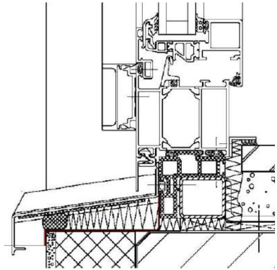
The air-tightness foil is marked in red in the section cut
