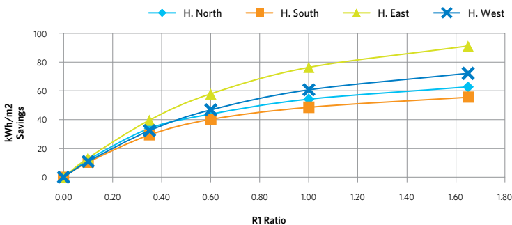
CHART 6.3.1.2 | KWH OF ENERGY SAVINGS PER GLAZING AREA DUE TO THE PROVISION OF HORIZONTAL SHADING DEVICE
