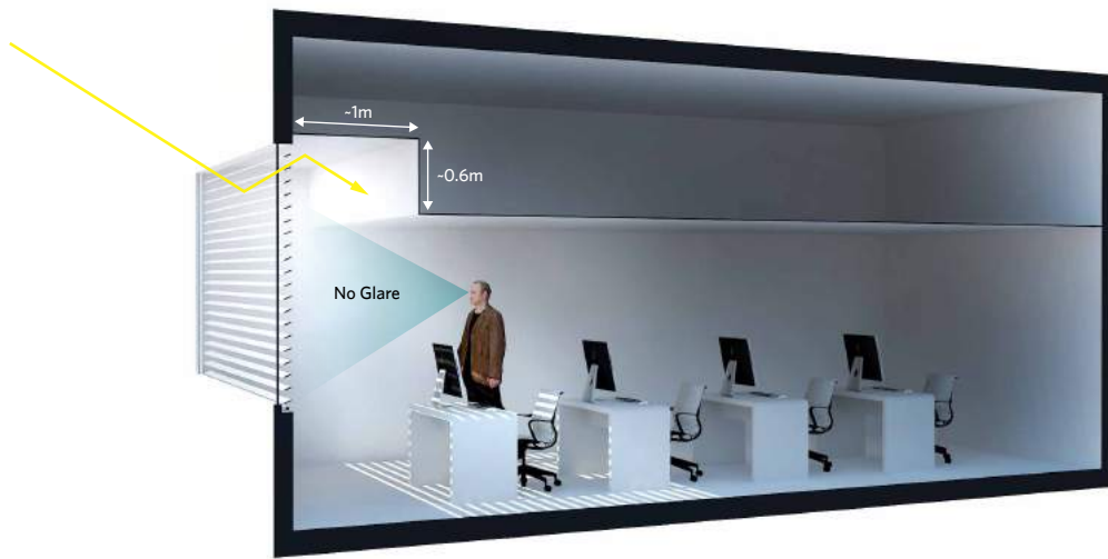
FIGURE 4.5.6 | DAYLIGHT DISTRIBUTION BLOCKED BY DROP OF FALSE CEILING BELOW THE TOP OF WINDOW HEIGHT
