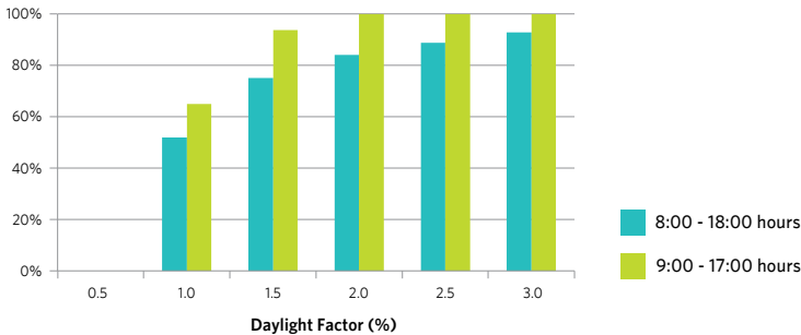
CHART 4.4 | PERCENTAGE OF HOURS WHERE THE DAYLIGHT FACTOR OF DIFFUSE LIGHT EXCEEDS 2,000 LUX LEVEL
