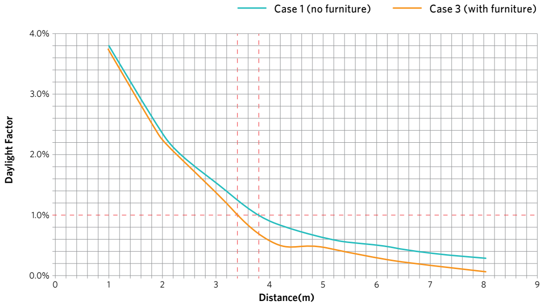
CHART 4.5 | DAYLIGHT LIGHT CURVE WITH AND WITHOUT FURNITURE
