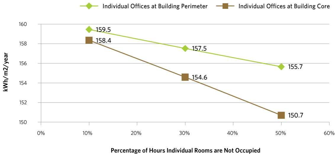
CHART 11.2 | BUILDING ENERGY INDEX OF VARIOUS CASE SCENARIOS
