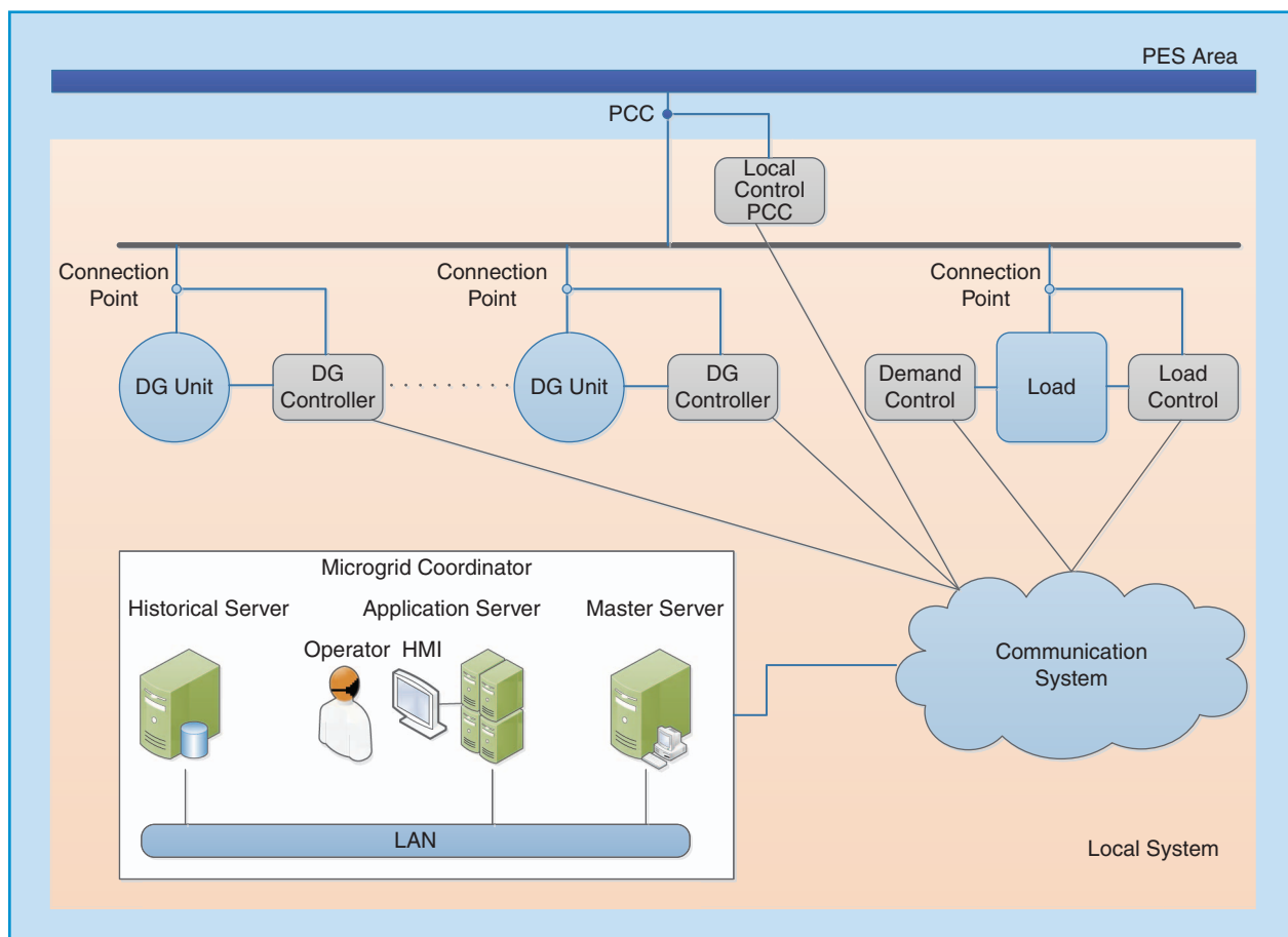
figure 7. Communications architecture of a microgrid.
