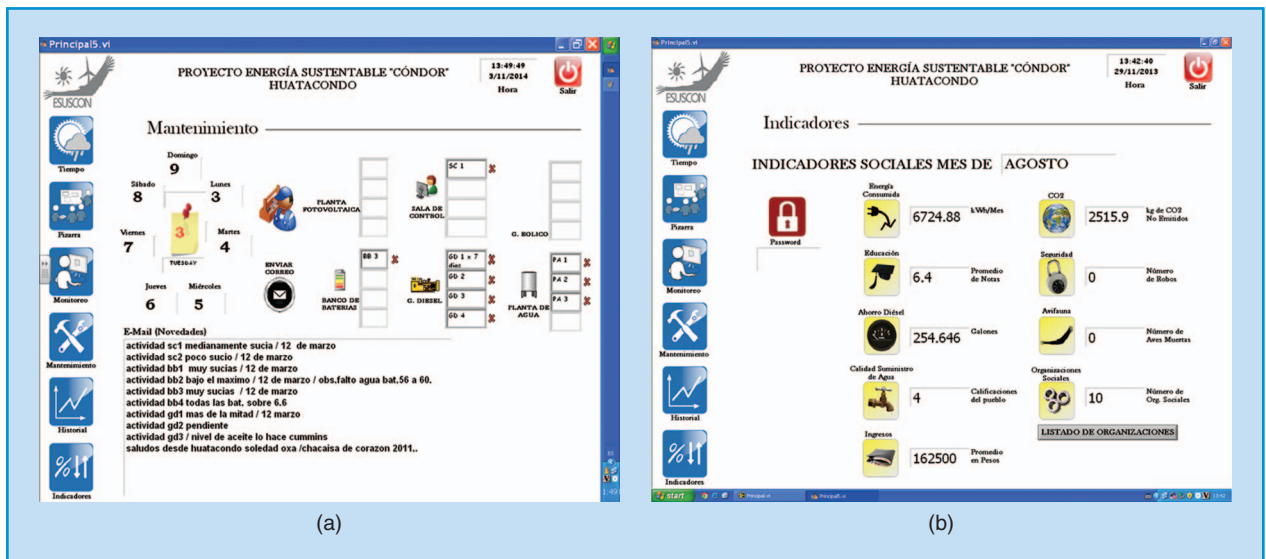
figure 9. The HMIs for (a) maintenance management and (b) sustainability indicators. The HMIs are presented in Spanish, as they were designed for the Huatacacondo community's use.
