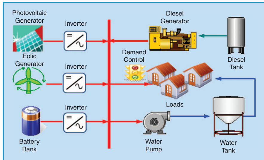
figure 8. A diagram of the Huatacondo microgrid.
